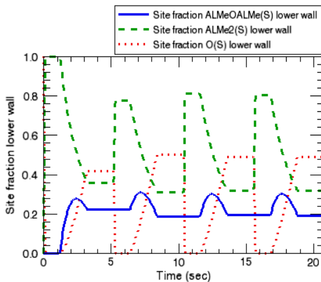
Figure 4 Time-dependent ALD Simulations—Stagnation-flow Site Fractions
