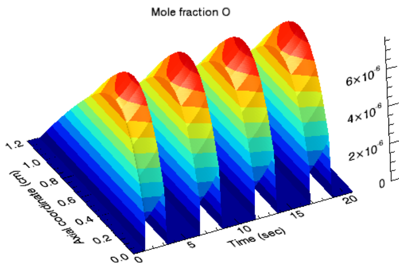
Figure 3 Time-dependent ALD Simulations—O Mole Fraction
